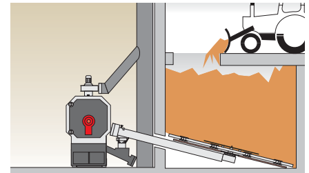
Bunker with rotary sweep extraction
